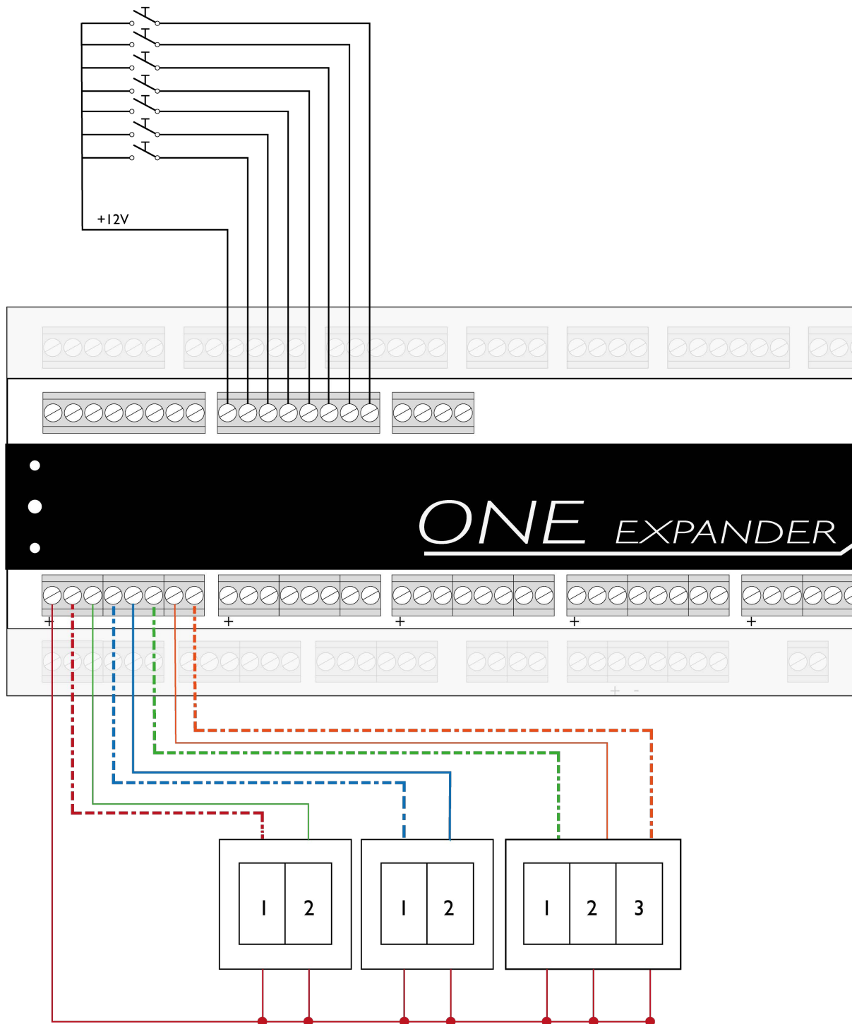
Figure 9. Inputs connection diagram
