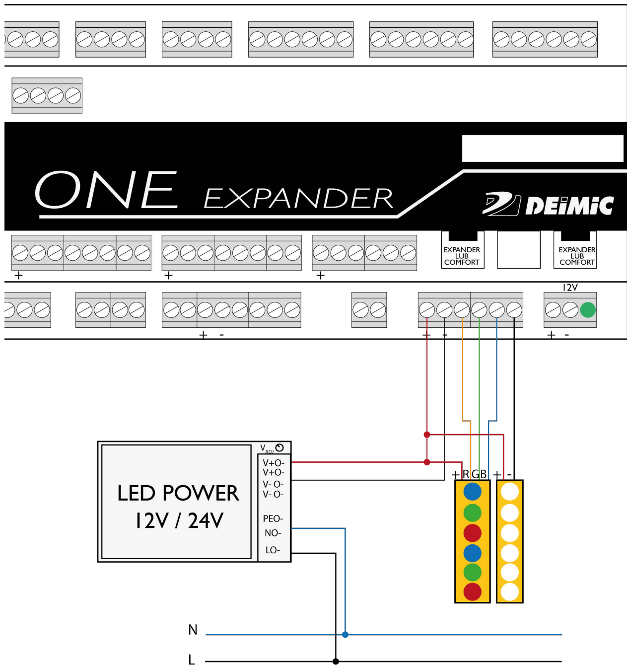
Figure 7. LEDs connection diagram – option 2
