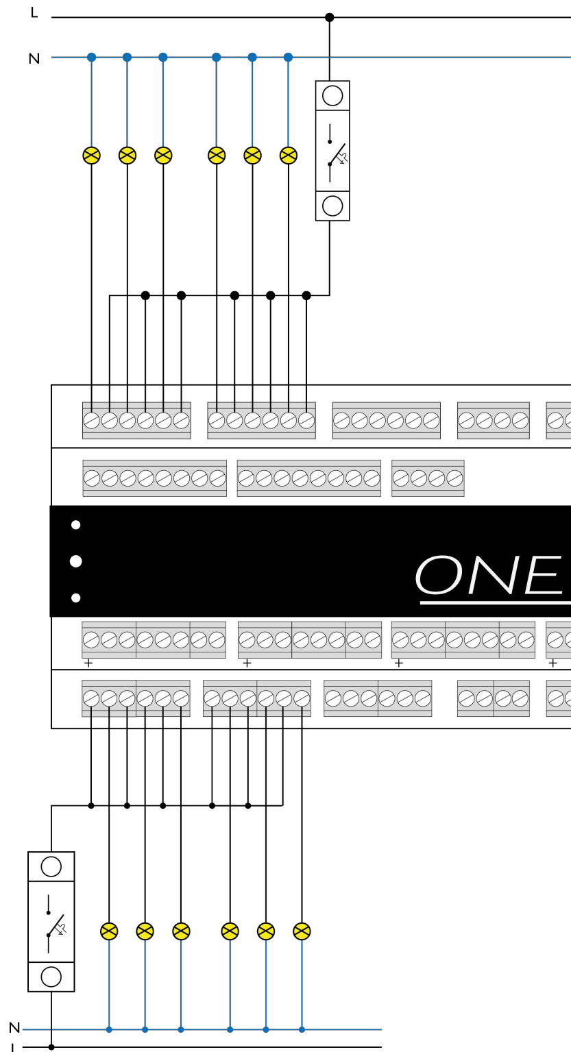
Figure 4. Lights connection diagram
