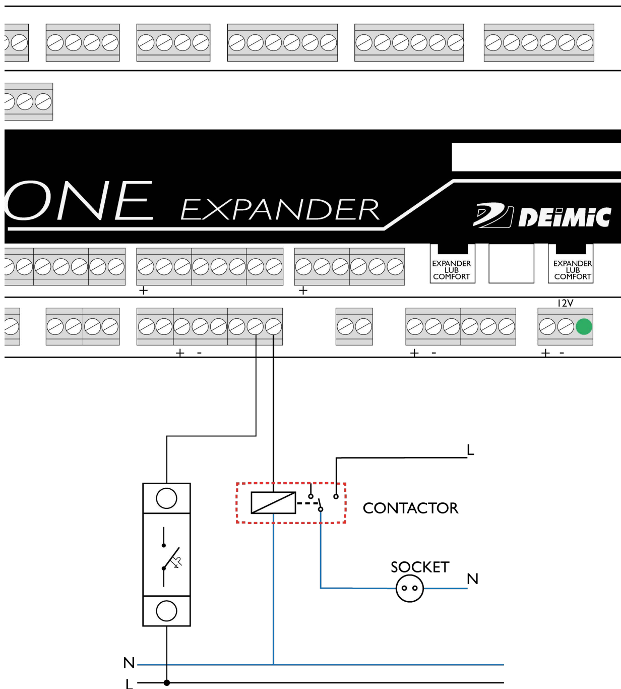
Figure 8. Contactors connection diagram
