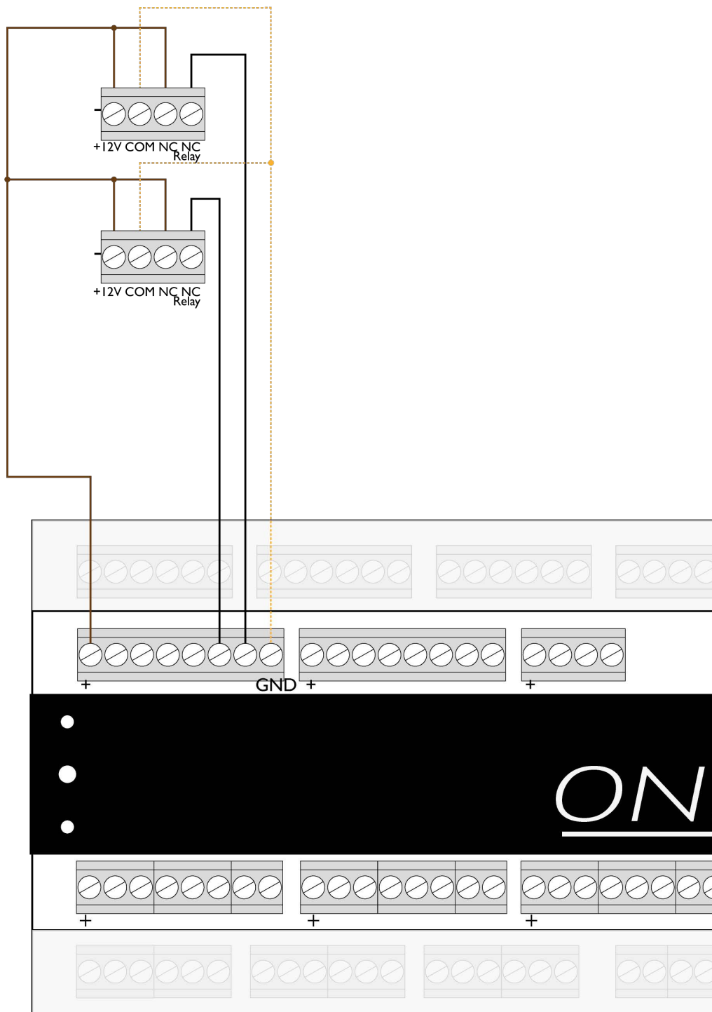
Figure 10. Motion sensors connection diagram
