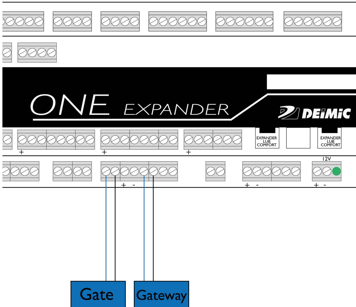
Figure 5. Gates and gateways connection diagram
